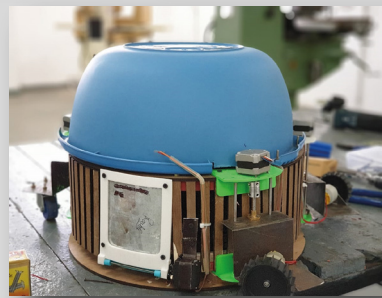
Pied Piper - Complete human touch free mouse trap device
